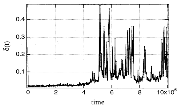
FIG. 5. The deviation of the locally averaged energies from the value of the equipartition. Individual energies are averaged over 20000 t_c around the given time t .
